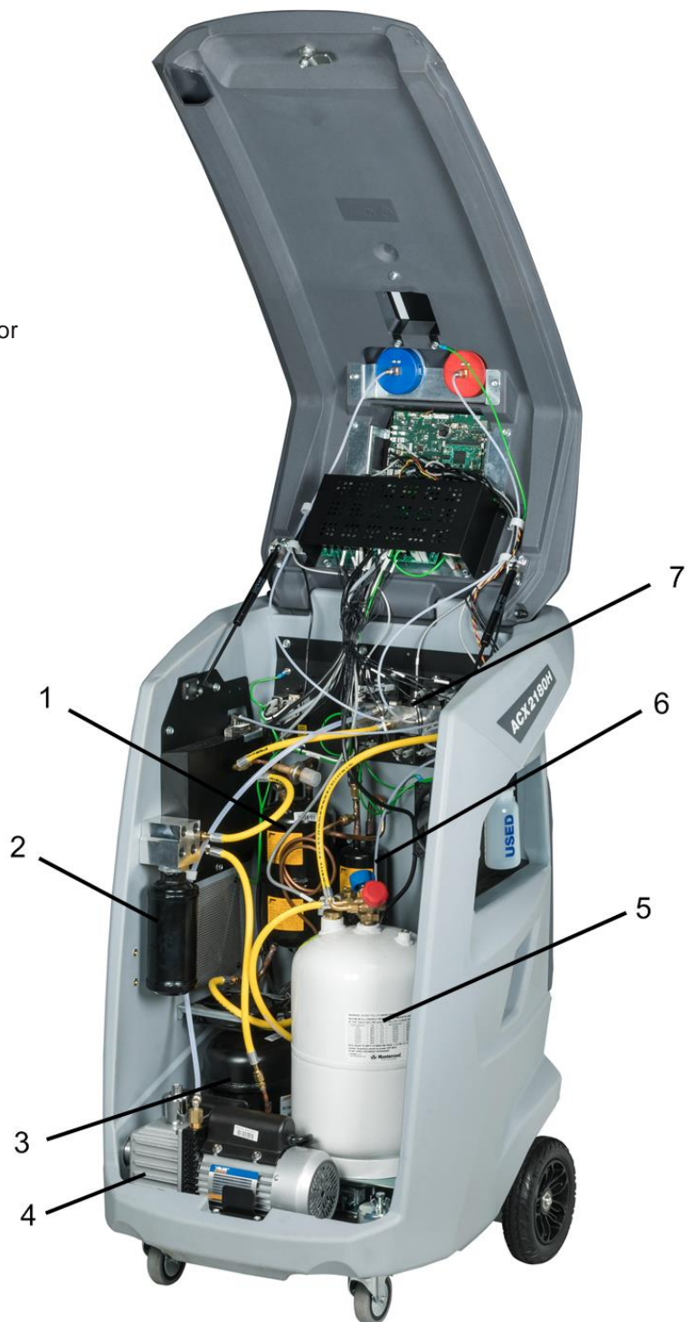
Fig. 4: Internal components
