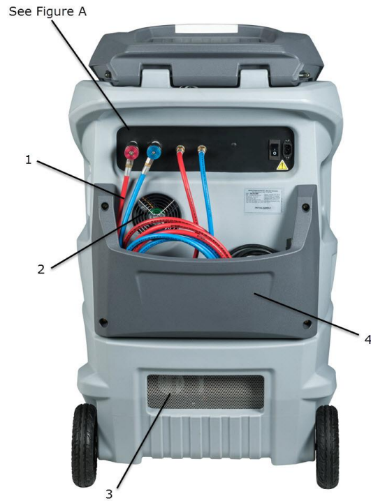
Fig. 2: Rear View
