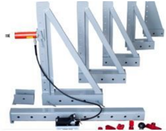
Multi Adapter Push Assembly
