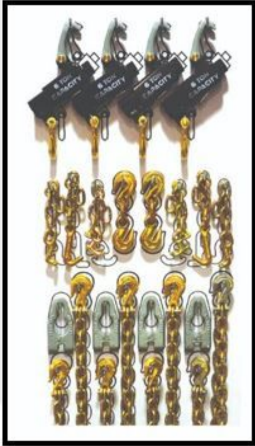
T4 Truck Tie Down
